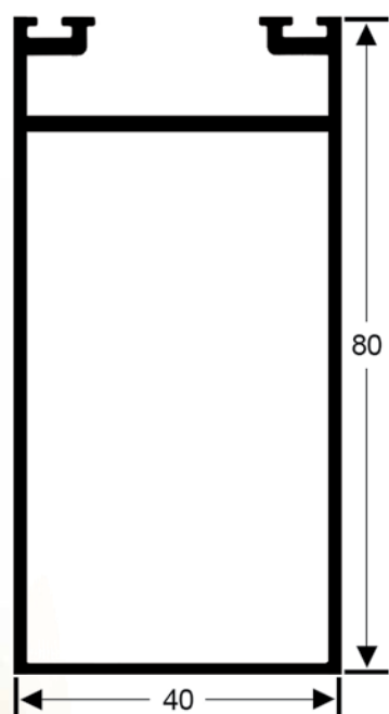
MC-72 | 1,109 kg/m
